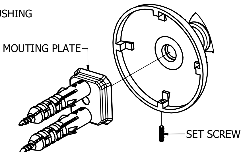
DETAIL D
