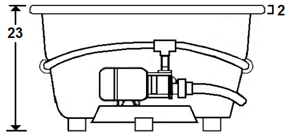
Standard Pump & Heater Location
