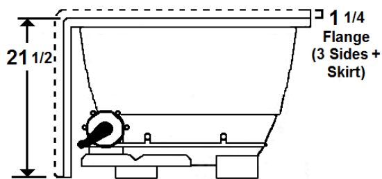
Standard (S) Blower & Heater Location
