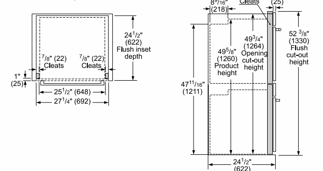
Flush installation Top view
