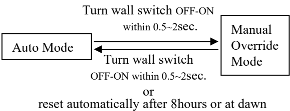
FIG.2 Manual Override Operating Diagram
