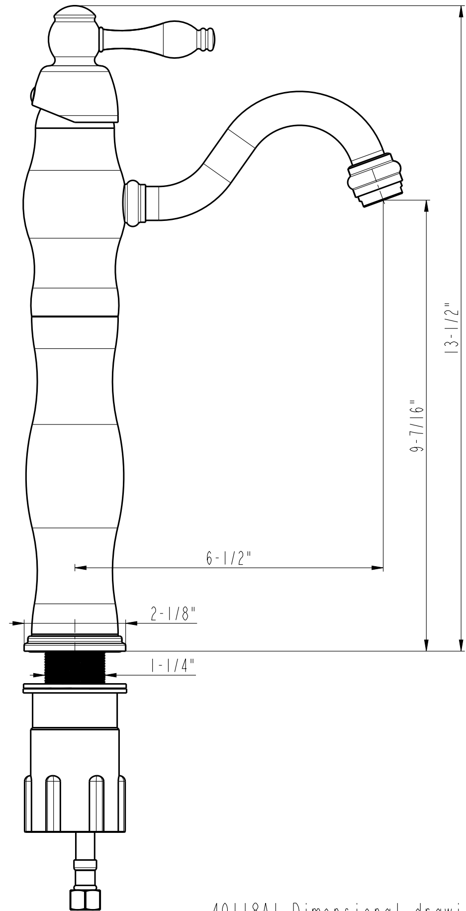
40118A1-Dimensional drawing
