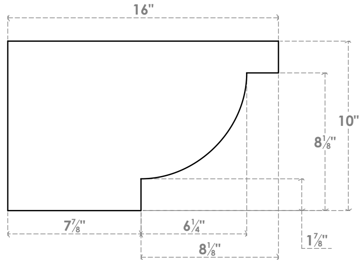
SIDE PROFILE
