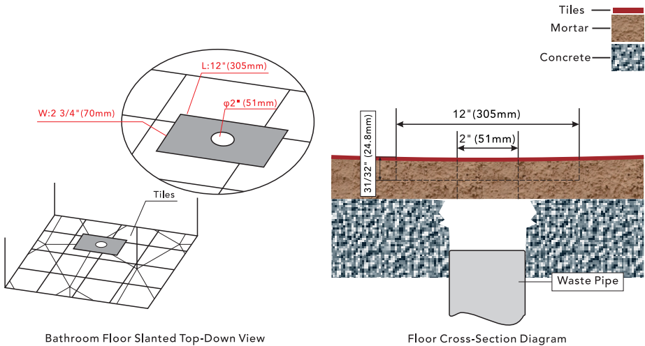
Bathroom Floor Slanted Top-Down View
