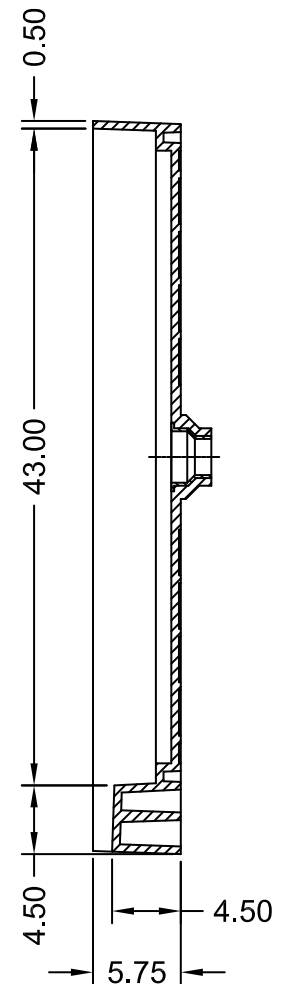
SECTION B-B
