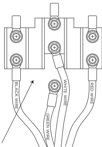
CUT OR REMOVE GROUND LINK
