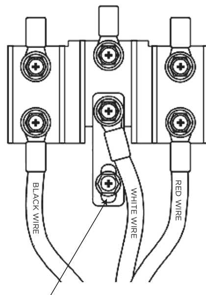
GROUND SCREW
