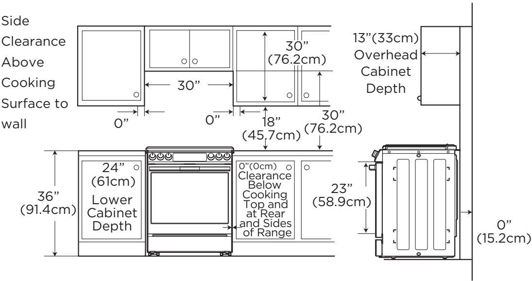
SLIDE-IN CUTOUT
