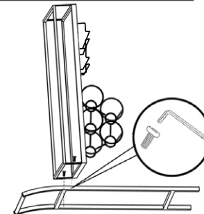
STEP 3 use parts B
