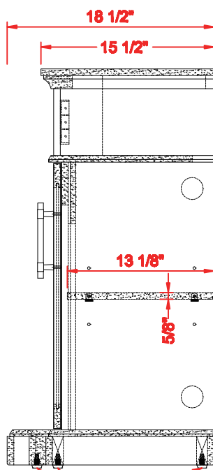
Adjustable Leveler
