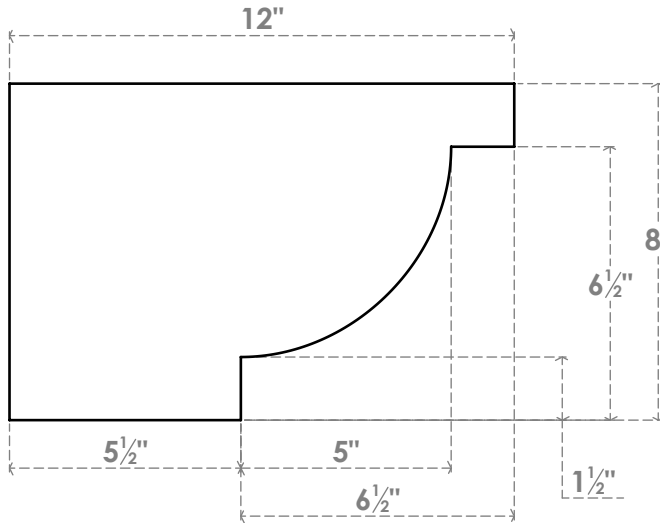
SIDE PROFILE
