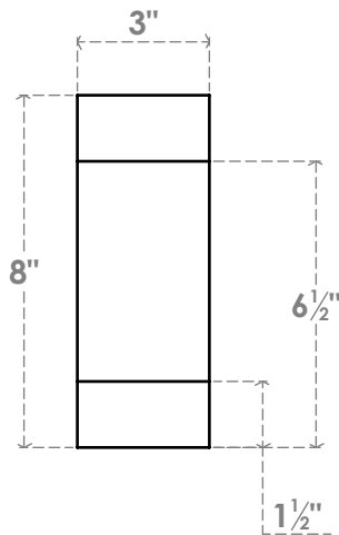
FRONT PROFILE
