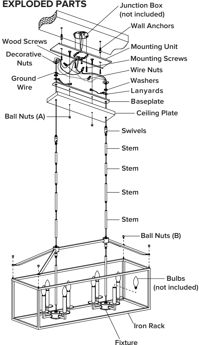
Decorative Nuts
