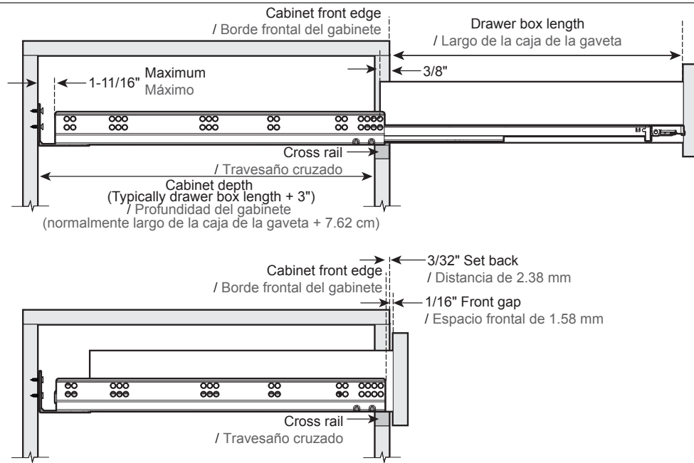
Face Frame / Marco frontal
