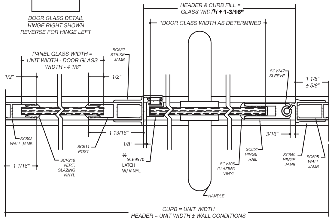
HORIZONTAL CROSS SECTION
