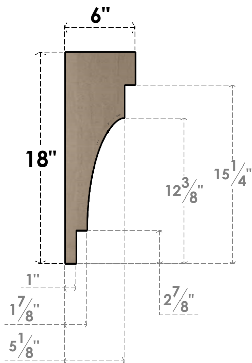
SIDE PROFILE
