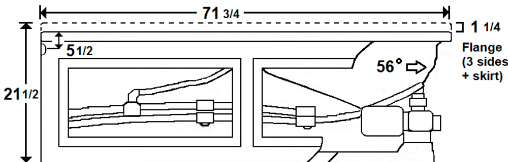
Standard (S) Pump w/ Heater Location
