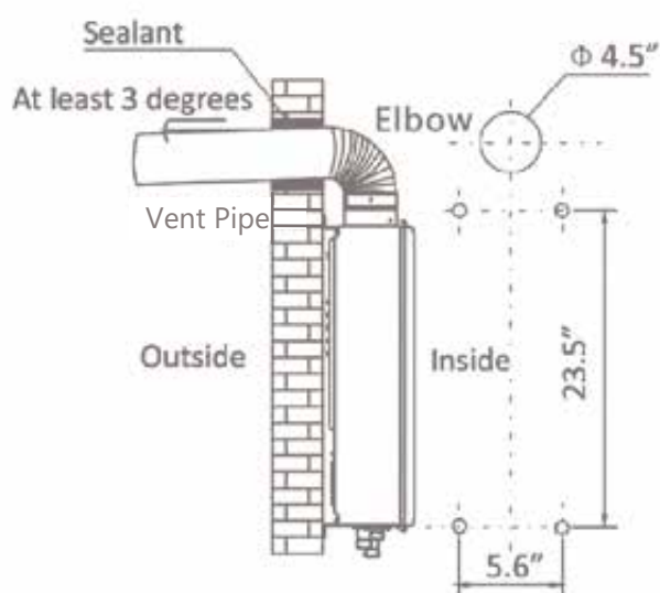
Back Installation
