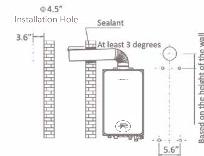
Side Installation
