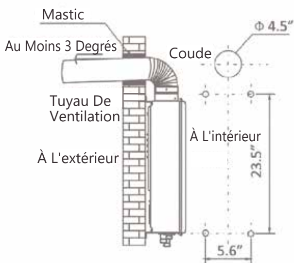
Retour Installation
