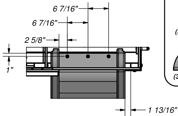
SLIDE HOLE DRILLING LOCATIONS
