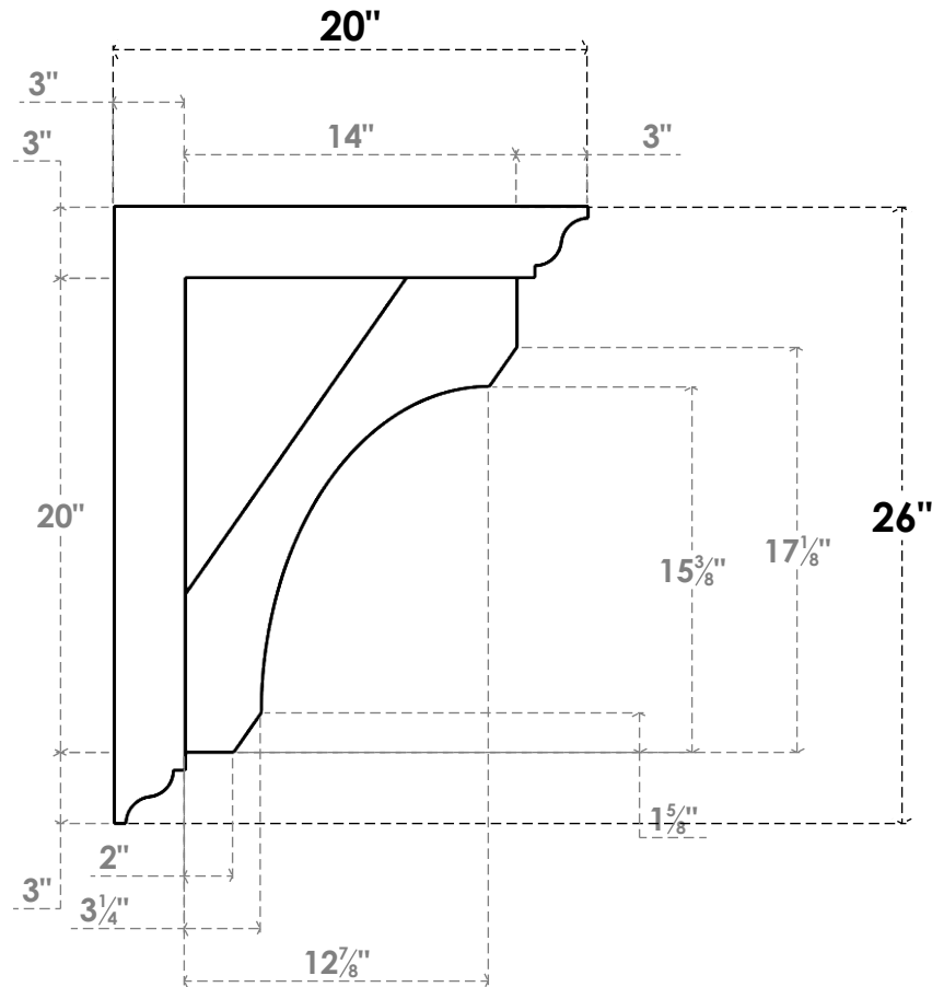
SIDE PROFILE
