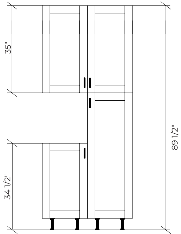
89 ½" tall cabinet with 35" wall cabinet
