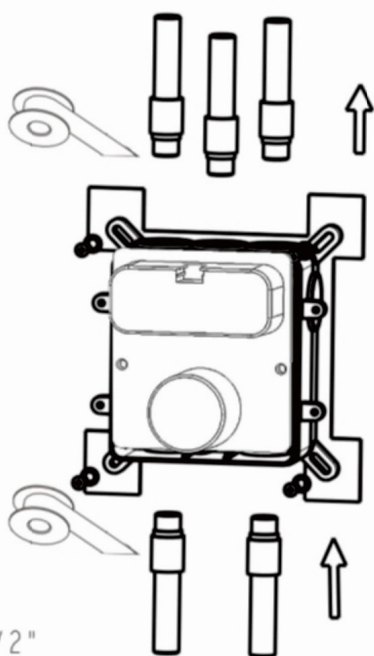
NPT 1/2" Mixed water outlet pipe
