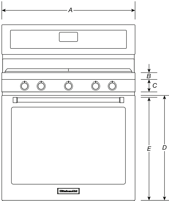
VISTA FRONTAL
