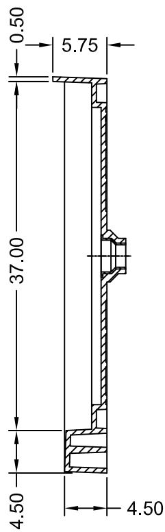
SECTION B-B
