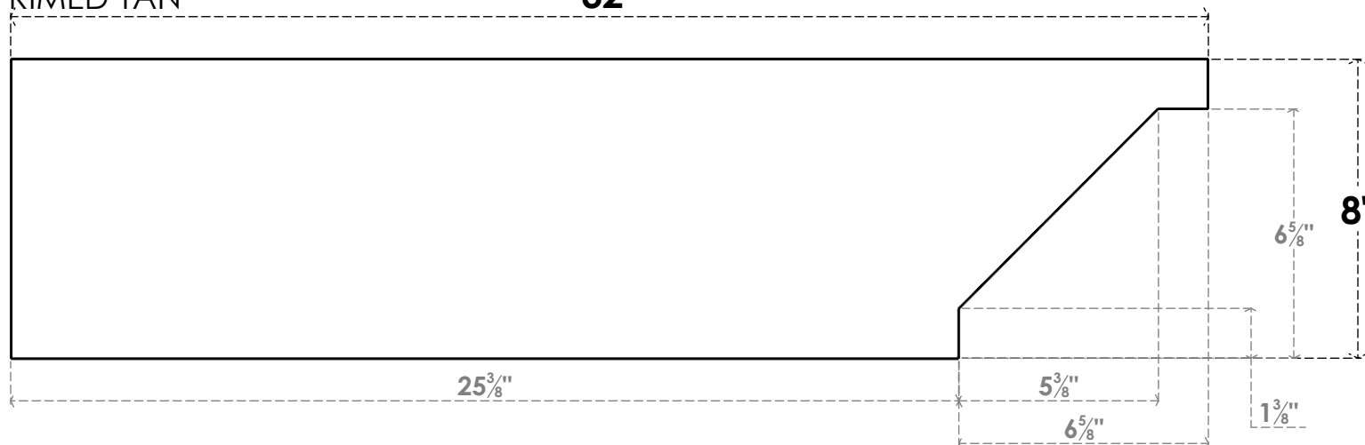
SIDE PROFILE
