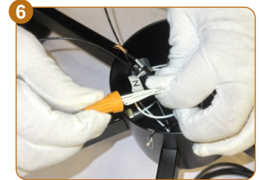
The white wire and the neutral wire are twisted together, while the black wire and the live wire are twisted together.
