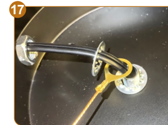
Install the grounding wire as shown in the diagram, ensuring that the grounding wire is clamped between two spacers.
