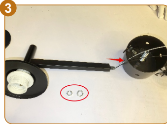
Remove the nuts and washers on the lamp base rod, and insert the wires and the rod into the holes..
