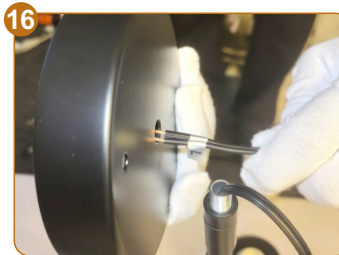
Thread the wire through the ceiling-mounted disc.
