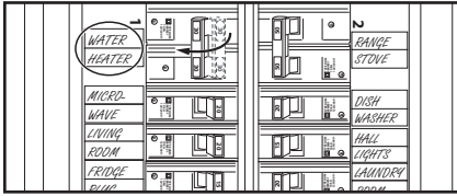
Figure 45 - Circuit Breaker.
