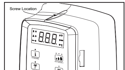
Figure 39 - Control Assembly
