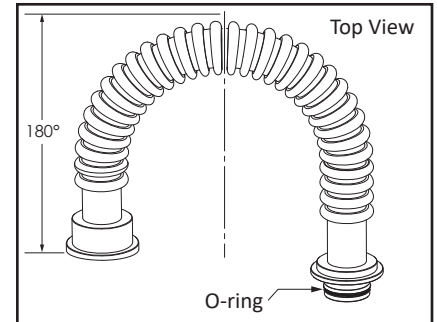
Figure 49 - Bend Flex Hose
