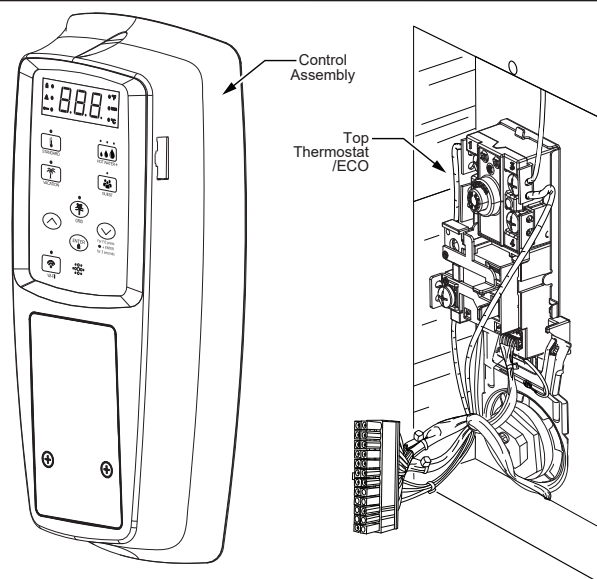
Figure 20 - Control Assembly
