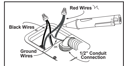
Figure 38 - Non-Contact Circuit Tester
