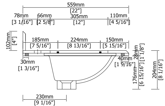
RIGHT VIEW
