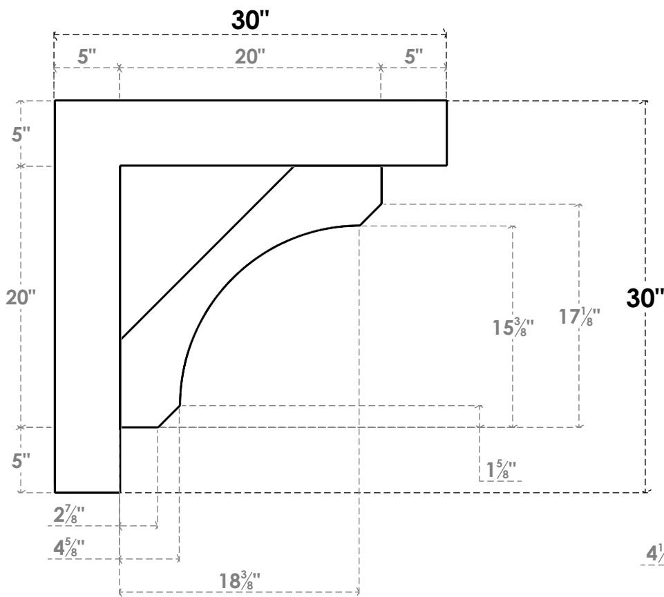
SIDE PROFILE
