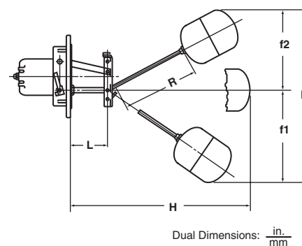
Figure 12: Float Position 3
