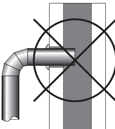
Stovepipe/Flue Connections
