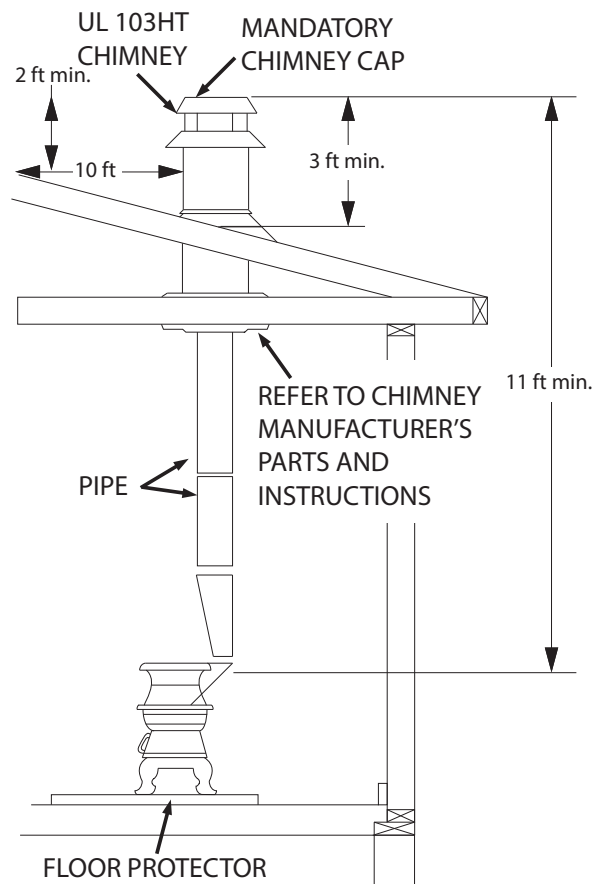
Chimney Construction Through Roof
