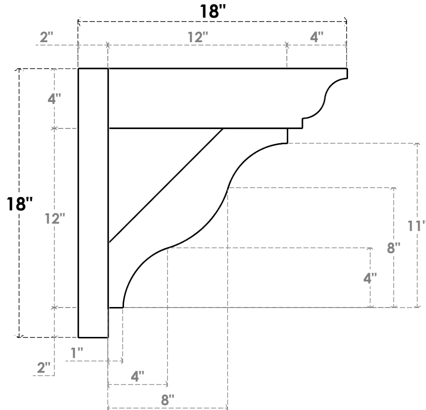
SIDE PROFILE
