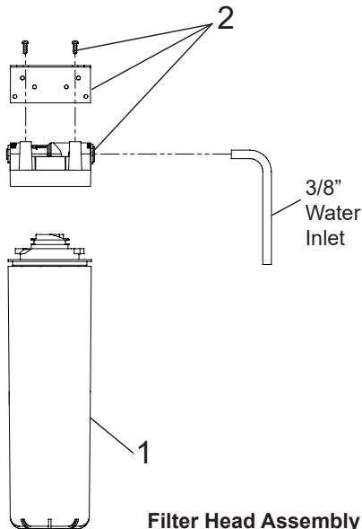
Filter Head Assembly used after 01/01/2021
