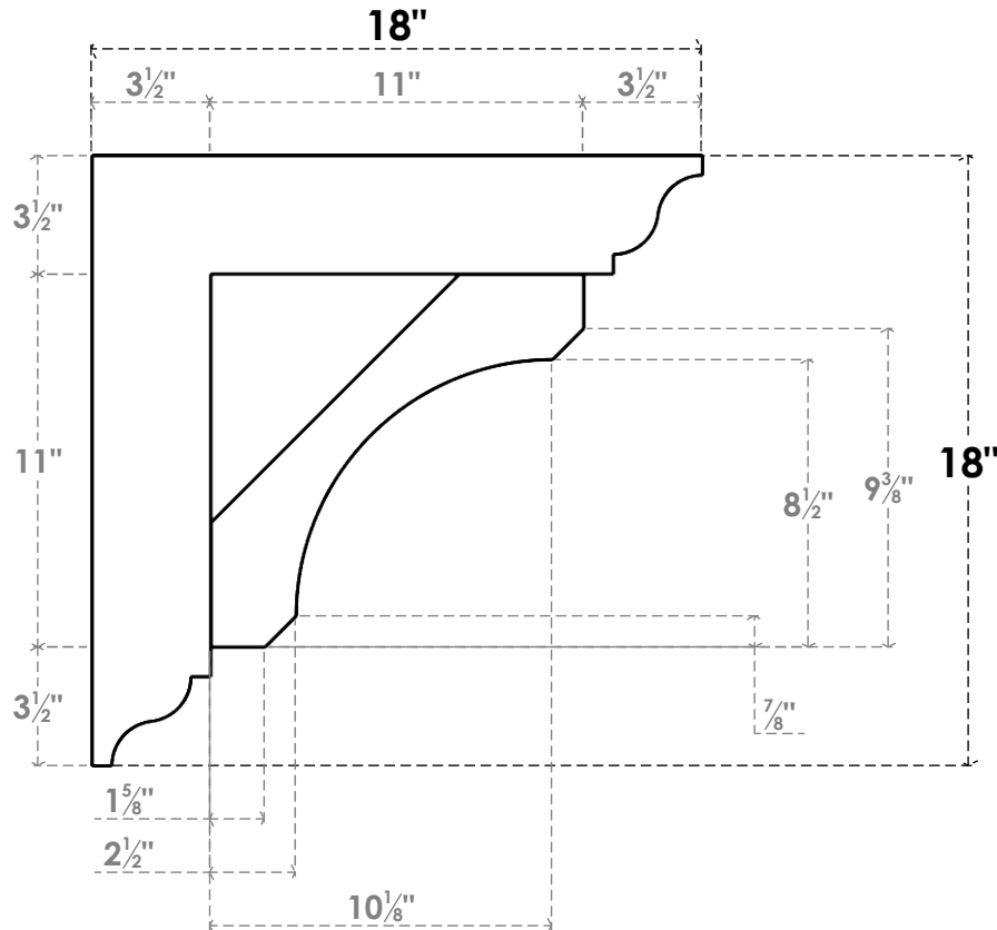
SIDE PROFILE
