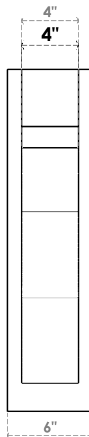
FRONT PROFILE
