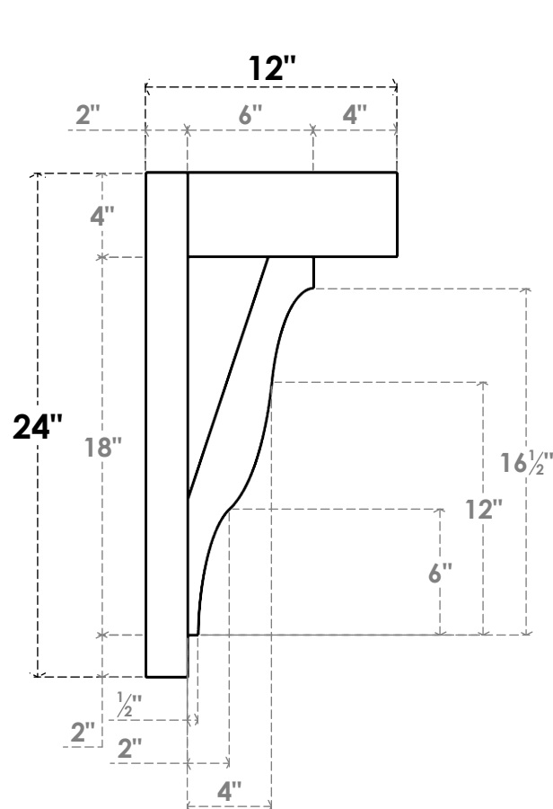
SIDE PROFILE
