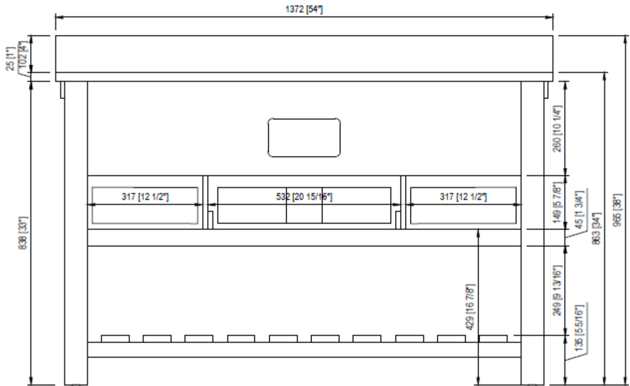
BACK VIEW
