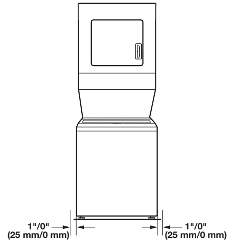
Side Clearances (recommended/minimum)
