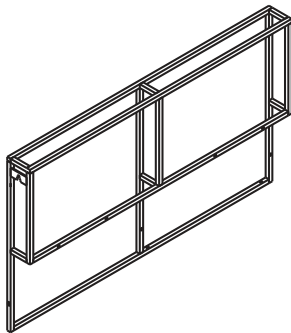
Right back frame (1 pc)
