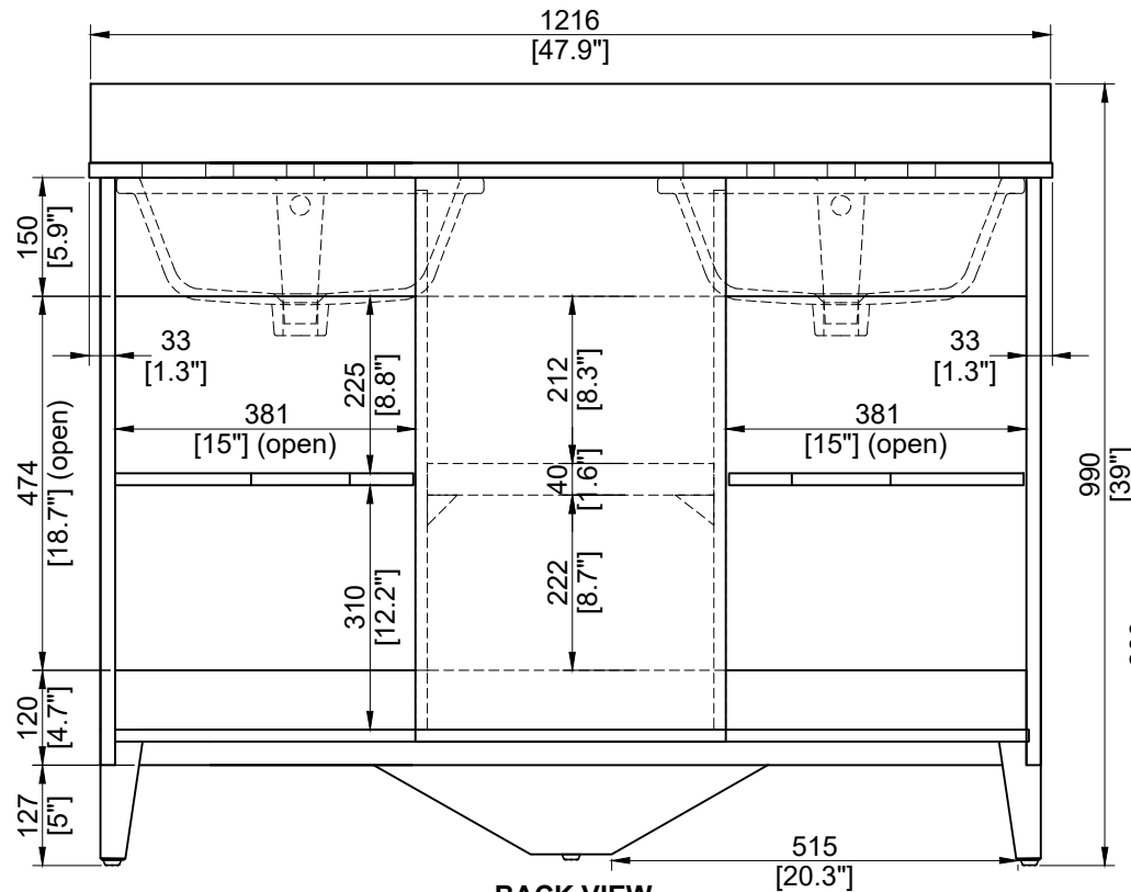
BACK VIEW
