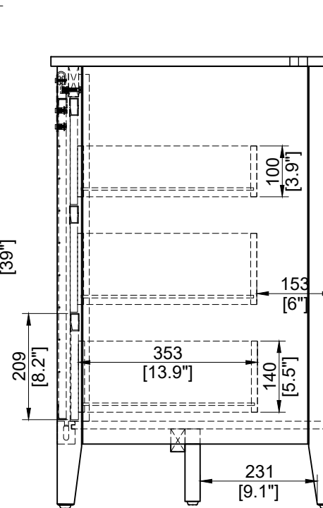
SIDE VIEW 2
