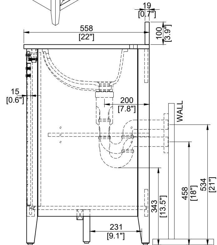
SIDE VIEW 1
