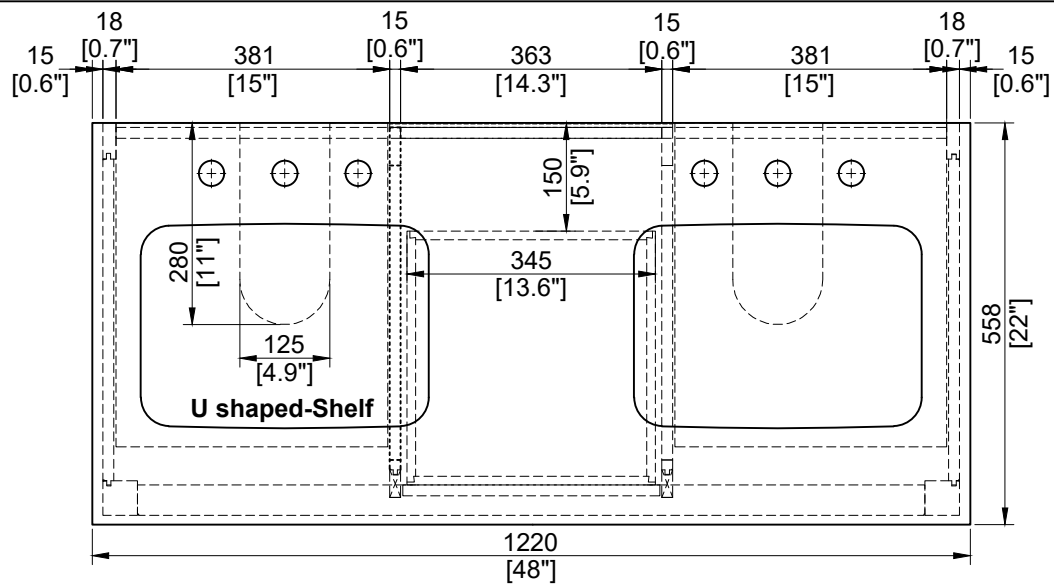
DETAIL VIEW
