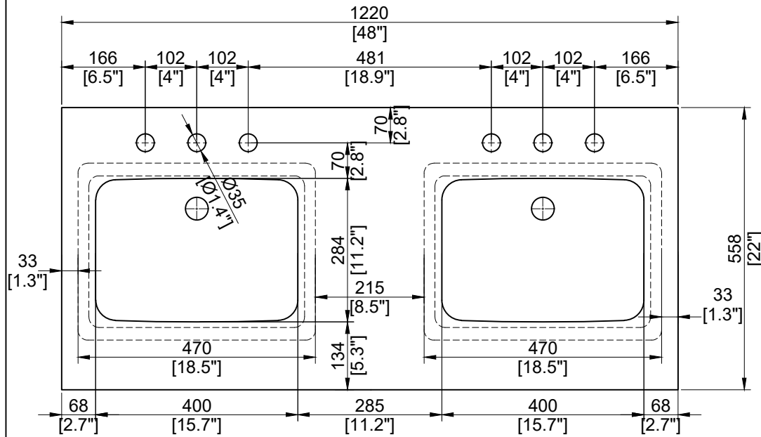
TOP VIEW
