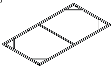
Stool Shelf Frame (1 pc)
