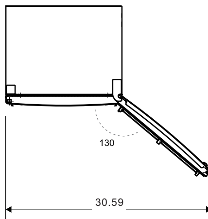
TOP OF REFRIGERATOR WITH DOORS OPEN 130
