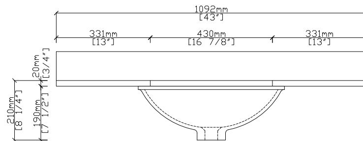
FRONT VIEW
