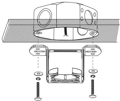
Octagon box
