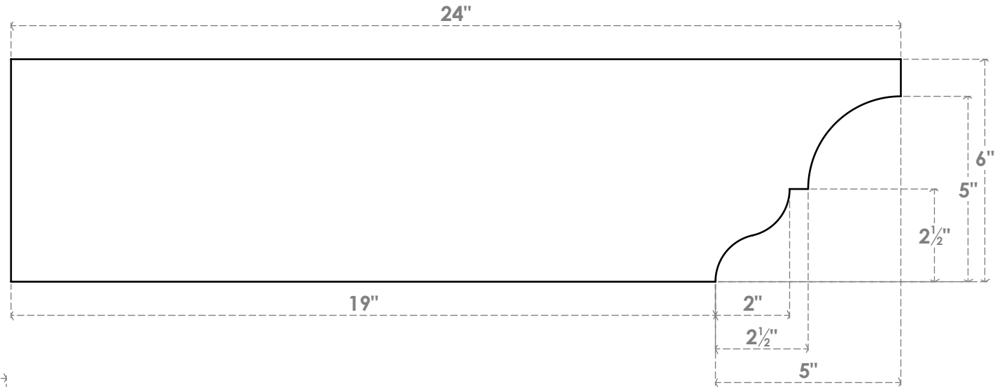
SIDE PROFILE
