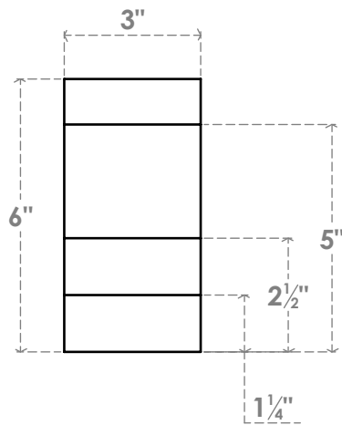
FRONT PROFILE
