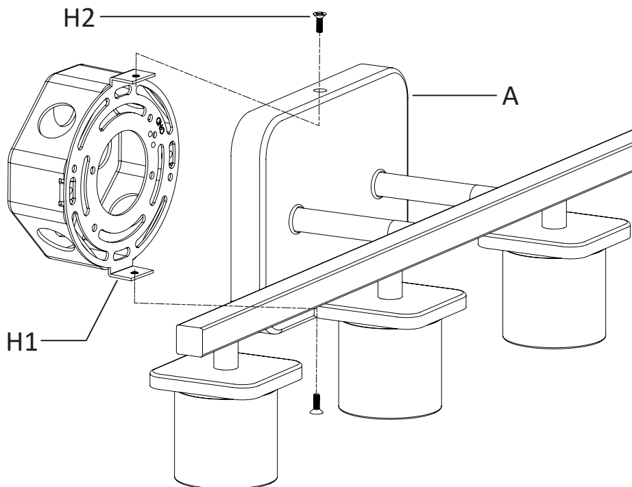
OPTION 1: Mount with glass shades facing down.
