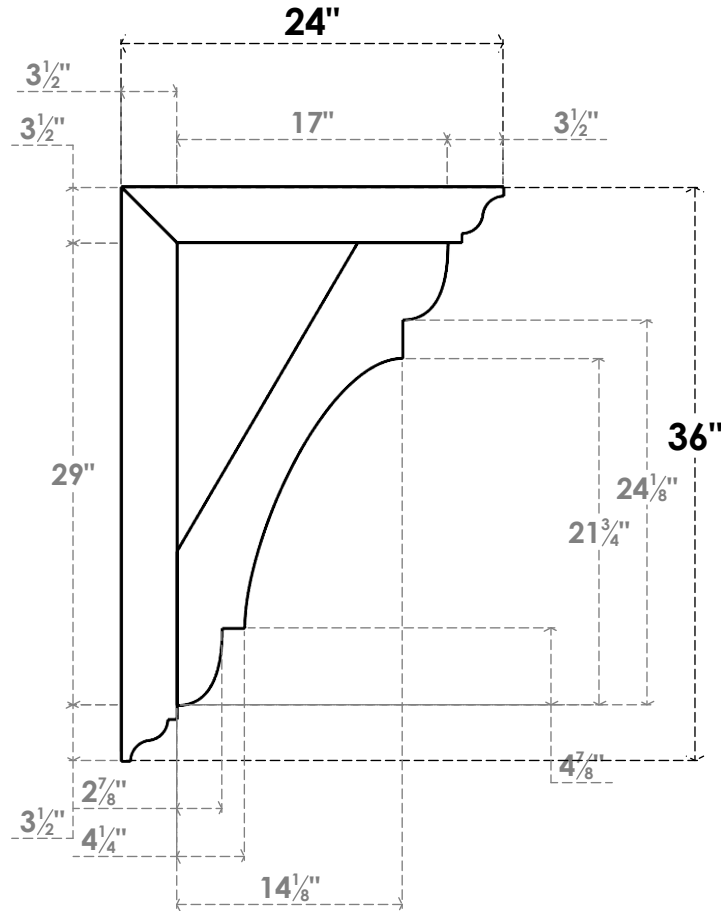
SIDE PROFILE
