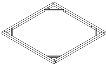
Seat frame (1 pc)
