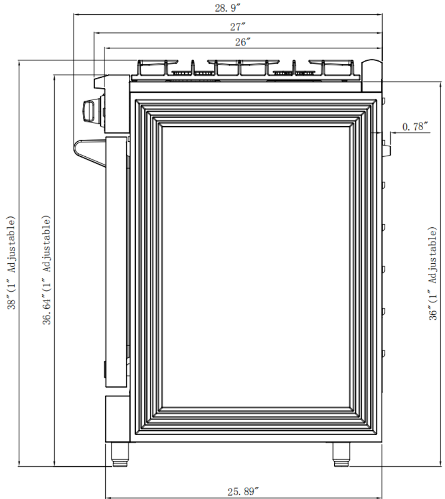
SIDE VIEW
