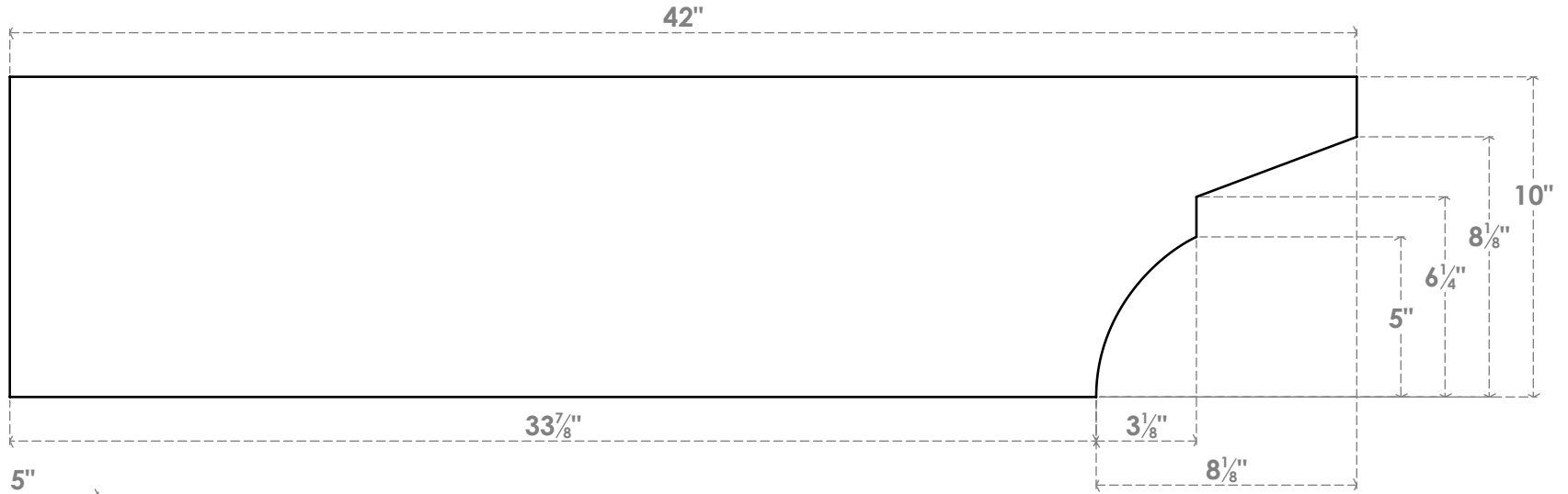
SIDE PROFILE
